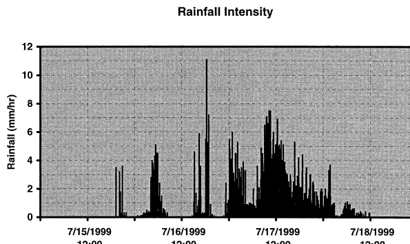
FIG. 6. Hourly rainfall intensity for the eight headwater rain gauges shows the periodic nature of the precipitation over the basin, with the most persistent precipitation at midday 17 Jul and the highest rainfall intensity on the 16th.
