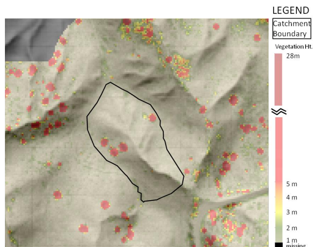
Figure 5. Aerial lidar-derived vegetation height over shaded topographic relief map.
