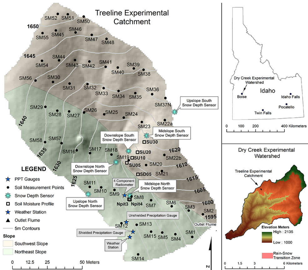
Figure 1. Location map of the Treeline experimental catchment in the Dry Creek experimental watershed and the location of instruments and measurement points.
