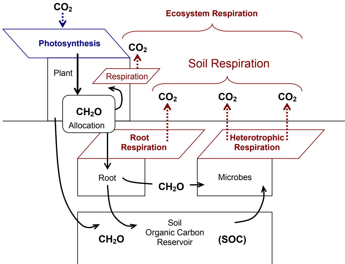
Figure 1.1. Terrestrial Carbon Cycle: C Storage and Exchange Processes
