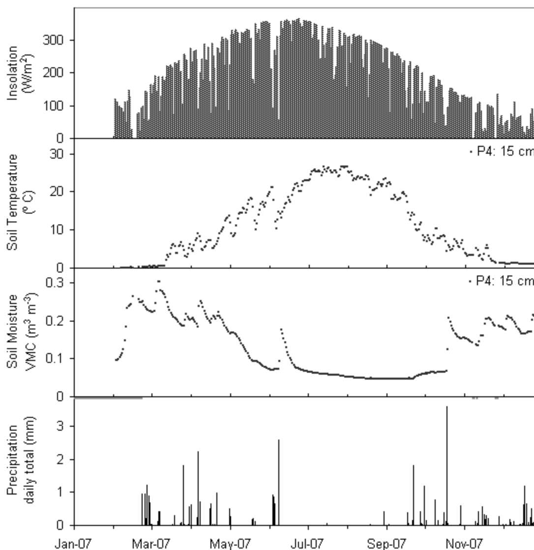
Figure 3.2. Upper Elevation Site 2007 Annual Climatic Trends (Days missing precipitation data indicated by gray blocks along top inside edge.)
