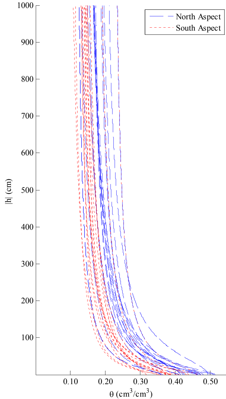
Figure 3.1: Soil water retention curves from the AMSO testing for the soils in this study. North aspect soils tend to have higher values of \theta at a given pressure head.
