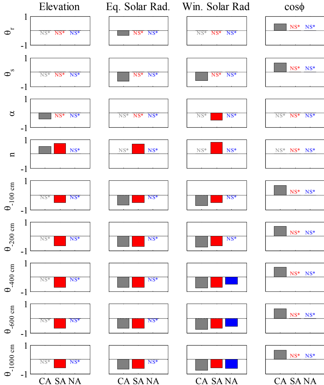
Figure 3.5: Spearman correlation coefficients relating elevation, fall/spring solar radiation, winter solar radiation, and \cos\phi to estimated van Genuchten parameters and \theta values for a range of pressure heads. NS* indicates that the Spearman correlation was not significant at the p < 0.05 level.
